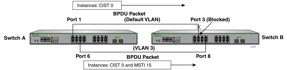
Figure 143. CIST and VLAN Guideline - Example 2
